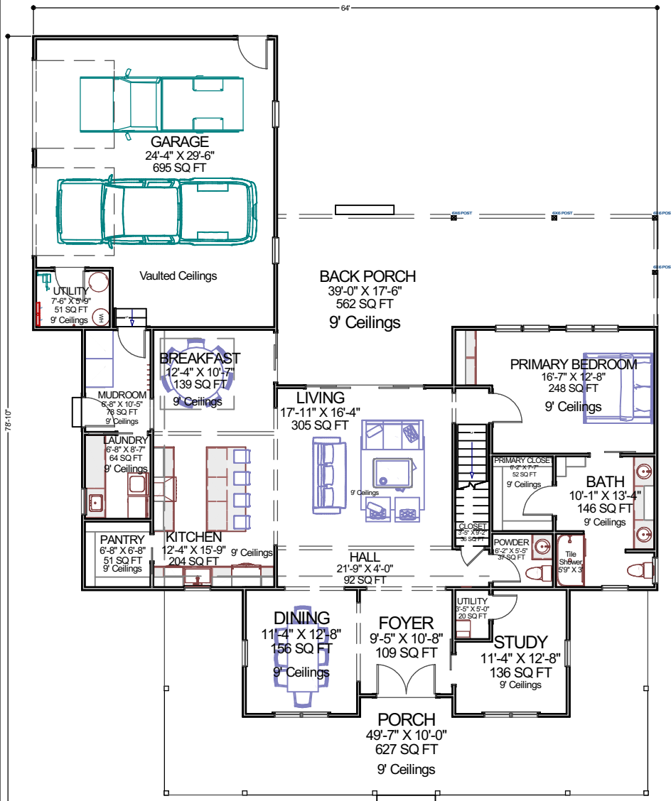
1st Floor
