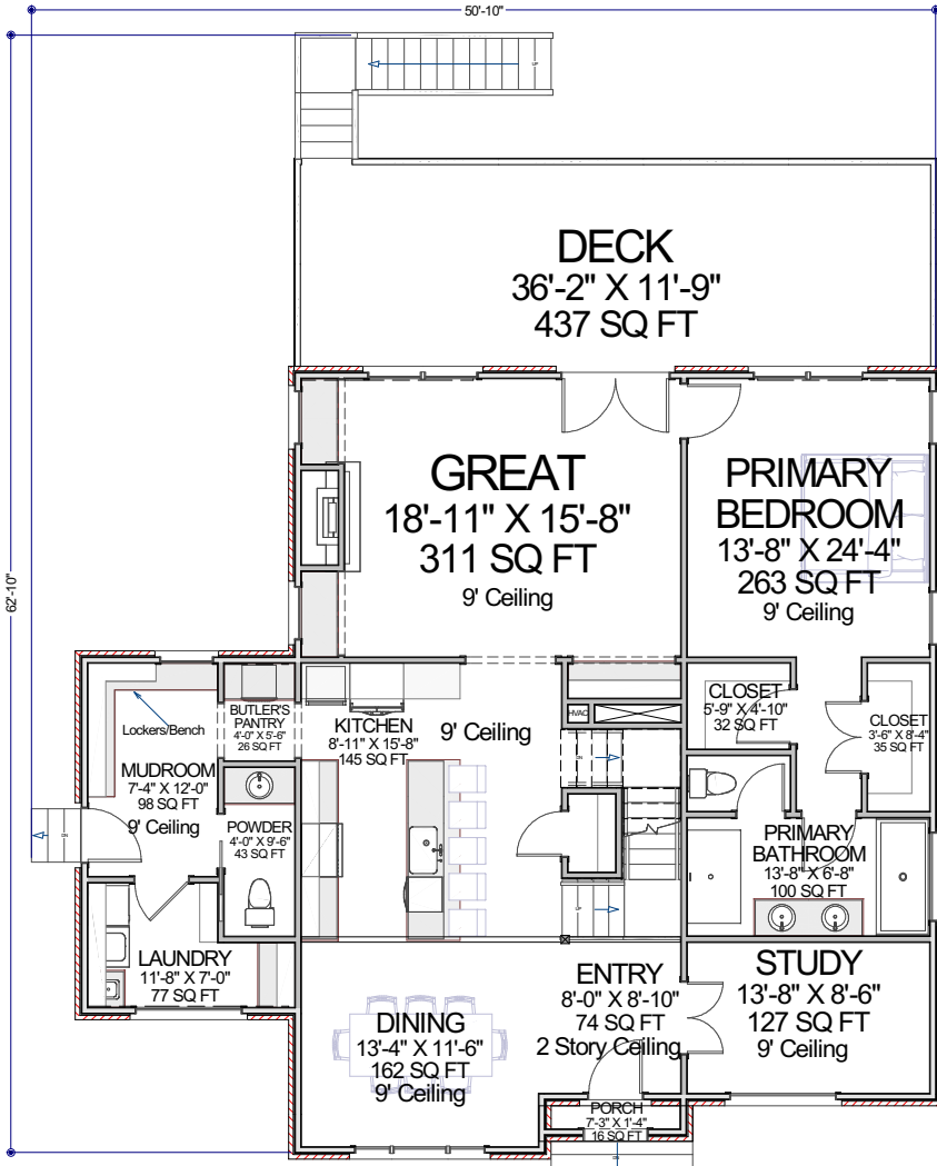
1st Floor
